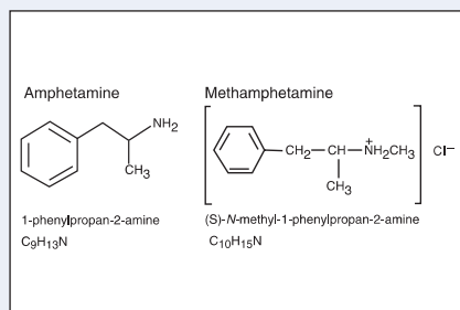
Figure 1: Chemical structures of amphetamine and methamphetamine (hydrochloride).
